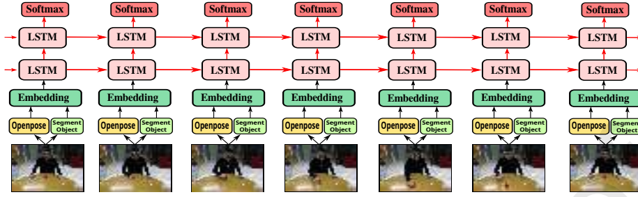
Figure 9: Proposed model architecture
