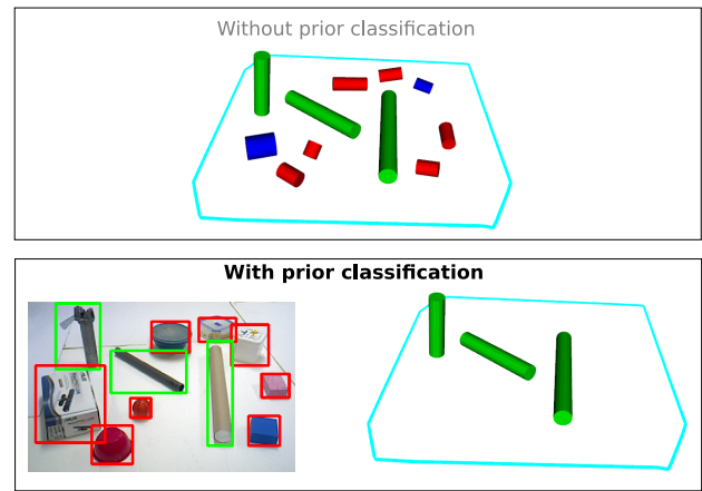
Fig. 12: Qualitative assessment of our framework with data acquired with an Asus Xtion 3D camera. Cylinder identification for an example scene. . Detection: Good and bad classifications in green and red, respectively. Parameter identification: green represents correct parameter estimation; blue represents correct non-cylindrical shape objects identified by the baseline quality of fitting criterion; red represents wrong estimations without the classifier.
