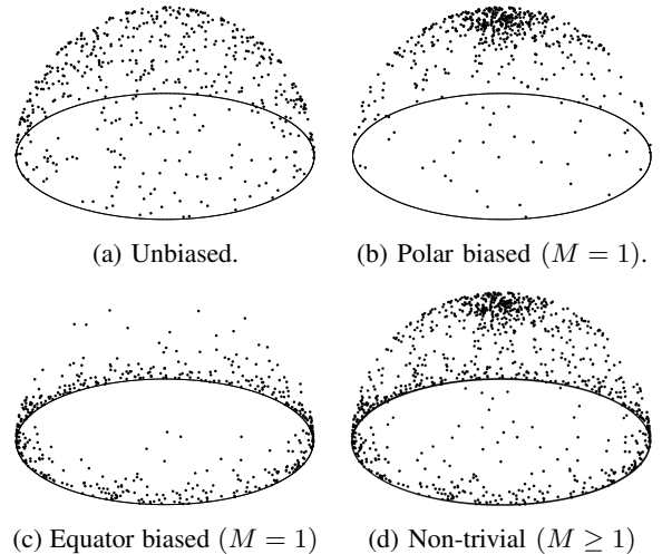
Fig. 3: Different sampled unitary spheres, where each point on the unit sphere represents the center of a candidate Voronoi cell orientation.
