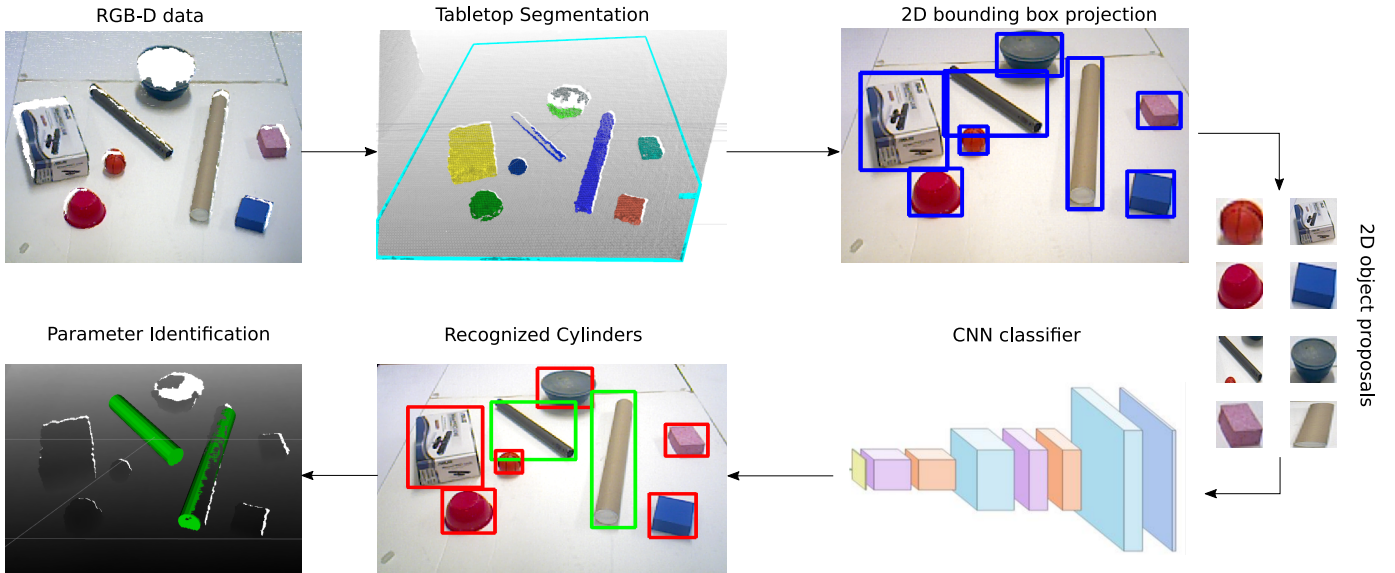
Fig. 2: General overview of our shape-based attention framework.
