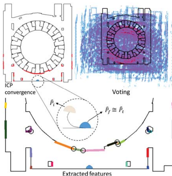
Figure 6: Simulation results for ITER map.
