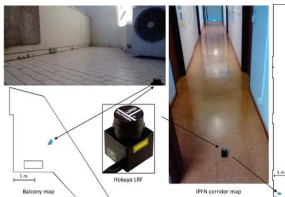
Figure 7: LRF sensor, photos and maps used in experimental testing.
