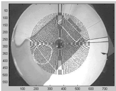
Figure 3: Image obtained by the catadioptric system with the 36 circles used to determine transition pixels.
