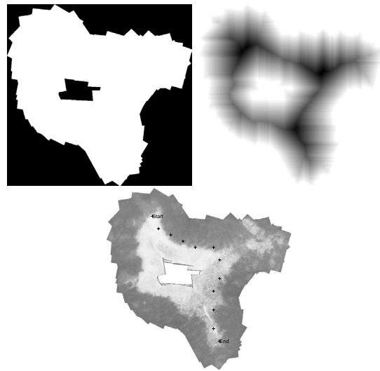
Fig. 8. Trajectory generation example – Valid mosaic region in white (upper left), cost image (upper right) and mosaic with superimposed trajectory (lower image).
