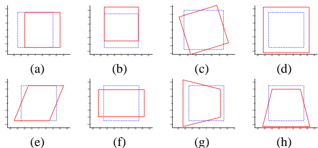
Fig. 2. Degrees of freedom of the planar projective transformation on images: (a) horizontal translation, (b) vertical translation, (c) rotation, (d) scaling, (e) shear, (f) aspect ratio, (g) projective distortion along the horizontal image axis, (h) projective distortion along the vertical image axis
