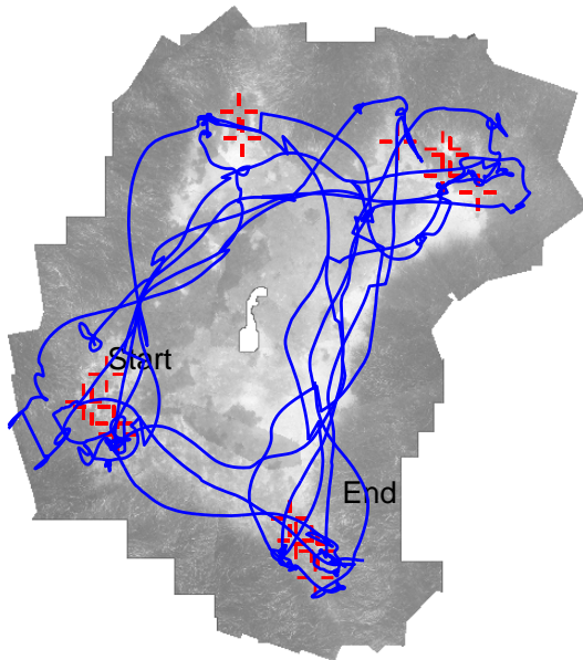
Fig. 11. Underwater mosaic servoing experiment. This plot shows a top-view of the ROV trajectory for the complete run with the reference positions marked with crosses. The ROV trajectory was recovered for the on-line image-to-mosaic matching with updates from the image-to-image tracking, and is marked with the full line.
