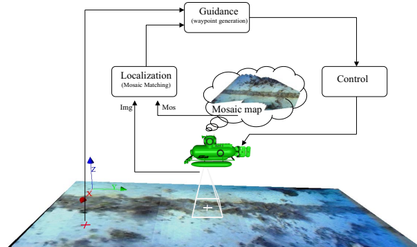
Fig. 7. Overall visual servoing control scheme.
