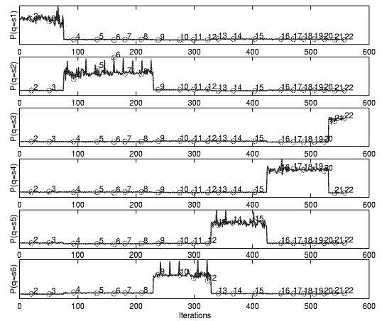
Figure 8: Log of probability localization in each state, with variance noise \sigma_1^2
