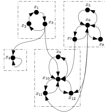
Fig. 2. Graphical representation of \mathcal{D}(A) : each rectangle represents an SCC and the two in the top are non-top linked SCCs.
