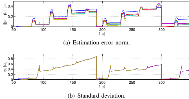
Fig. 1. Estimation error and standard deviation of the first 5 landmarks.
