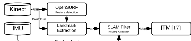
Fig. 5. The full algorithm used in the experiments.
