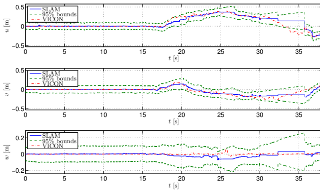
Fig. 7. Time evolution of the real and estimated velocity
