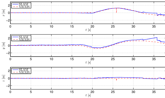
Fig. 6. Time evolution of the real and estimated trajectory
