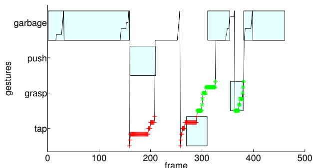
Figure 10: An outcome of the human-robot manipulation scenario showing the limitations of our approach in the presence of noise: the Push-Tap-Grasp action sequence performed by the user is not correctly classified by the statistical model. Red plus signs: tap states, green stars: grasp states, blue crosses: push states, rectangles: human-labeled ground truth segmentation.
