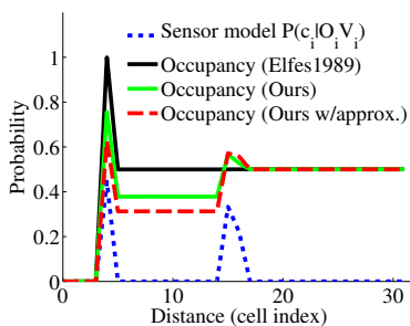
Fig. 4. Occupancy along a 1D ray given Elfes’ formulation and our formulation with and without approximation (9)
