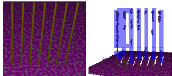
Fig. 5. Virtual scenario with vertical bars to induce similar cost minima (left); resulting occupancy grid in our whole-cost-curve approach (right). Occupied cells are marked with blue. Result should be 7 parallel bars.
