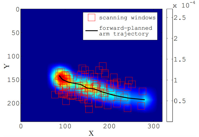
Figure 3. Nonuniform image processing based on a manipulation-relevance saliency. The black line corresponds to a mentally-simulated (forward-planned) arm trajectory that is projected to the image plane of a stereo camera. The heat-map corresponds to an intensity of the saliency function. The red rectangles are scanning image windows, for which visual features are computed. The anchors of the scanning windows are sampled with respect to a saliency function, i.e. more dense visual scanning is done where the relevance function has higher values, and less dense scanning where it has low values. The plot corresponds to the right stereo camera. The same procedure is done for the left camera.
