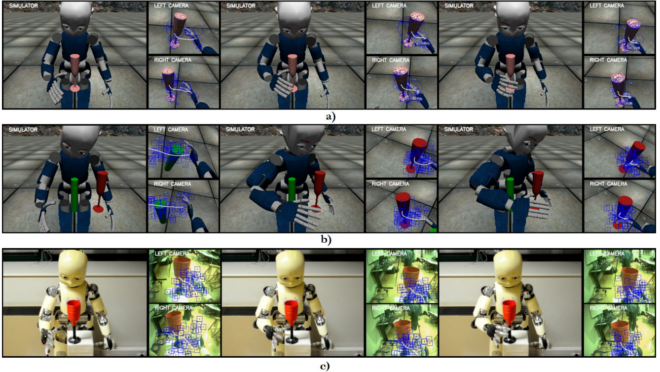
Figure 4. Experiments of visually-guided reaching and grasping in the iCub’s simulator, in two different scenarios with two detectors, and with the real robot. Visual computation is in every cycle of the of the control loop distributed to manipulation-relevant spatial locations of the stereo images. Figures show execution of eye-arm-hand coordination from the start of the task (left) until the successful grasp completion (right). The white line corresponds to a mentally-simulated arm trajectory that is projected to the image planes of stereo cameras. The top row of figures (a) corresponds to the no-obstacle scenario with SURF detector. The blue circles correspond to detected strong feature points. The middle row (b) corresponds to the obstacle scenario with histogram-based detector. The blue rectangles are scanning image windows, for which visual features are computed. The bottom row (c) corresponds to the no-obstacle scenario with histogram-based detector with the real robot. Figures show execution of eye-arm-hand coordination from the start of the task (left) until the successful grasp completion (right).
