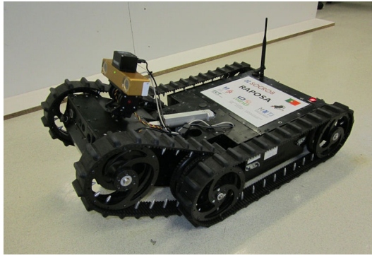
Fig. 1. RAPOSA-NG.
