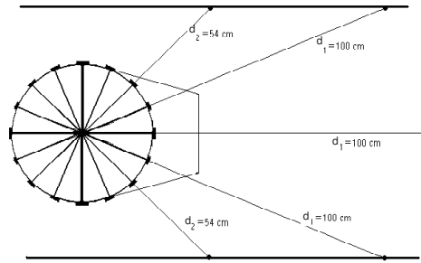
Fig. 2. Expected sonar measurements when traveling near a wall.
