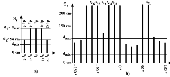
Fig. 3. a) Mask with the geometric configuration of the sectors; b) Typical Polar Histogram, showing the set S_c of sector candidates.
