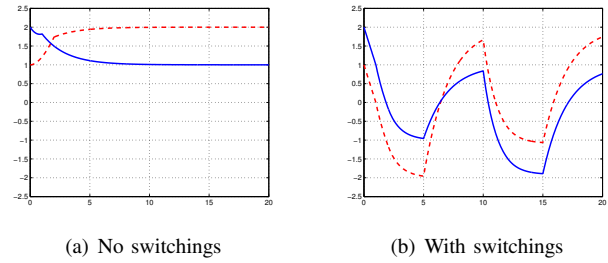
Fig. 3. Synchronization with non-homogeneous delays \tau_1 = 2[s] , \tau_2 = 1[s] , v_L = 1[s^{-1}] . Solid line - \gamma_1 - \gamma_2 ; Dash line - \gamma_1 - \gamma_3
