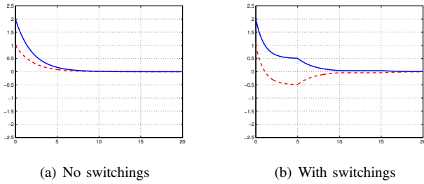
Fig. 1. Synchronization with no time delays, v_L = 1[s^{-1}] . Solid line - \gamma_1 - \gamma_2 ; Dash line - \gamma_1 - \gamma_3
