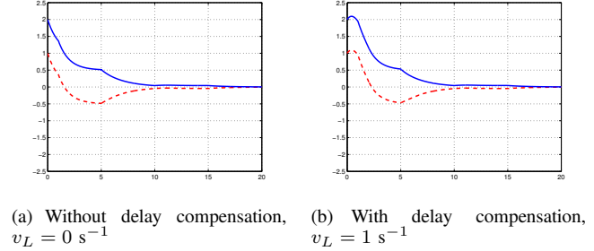
Fig. 4. Synchronization with non-homogeneous delays \tau_1 = 2[s] , \tau_2 = 1[s] . Solid line - \gamma_1 - \gamma_2 ; Dash line - \gamma_1 - \gamma_3
