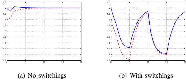
Fig. 2. Synchronization with homogeneous delay \tau = 2[s] , v_L = 1[s^{-1}] . Solid line - \gamma_1 - \gamma_2 ; Dash line - \gamma_1 - \gamma_3
