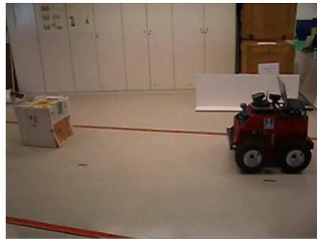
Figure 2: The HANS vehicle (ATRV robot) in the test environment; note the obstacle ahead in the "road"
