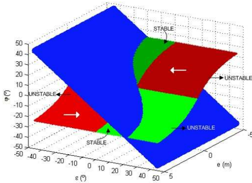
Figure 7: Lyapunov analysis
