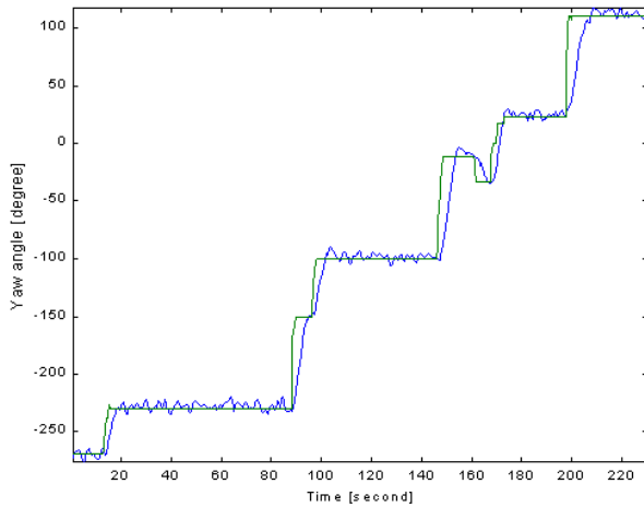
Fig. 4. Yaw command and vehicle response.
