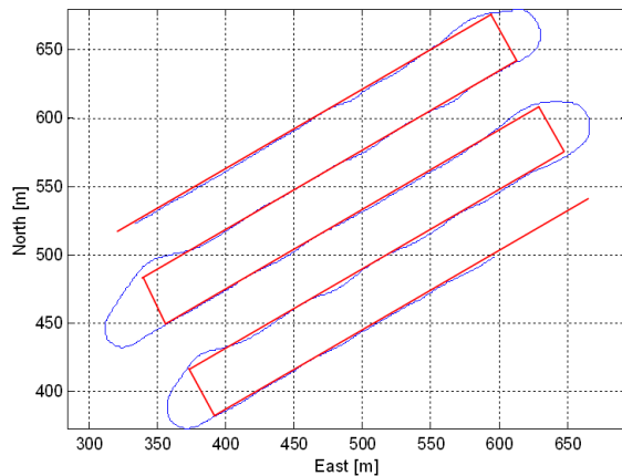
Fig. 5. Reference and actual vehicle paths.
