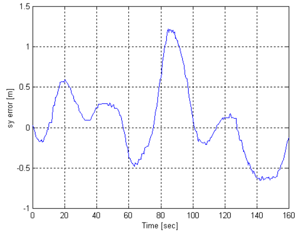
Fig. 6. Path following error.
