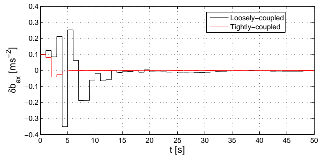
Figure 9: Bias misalignment
