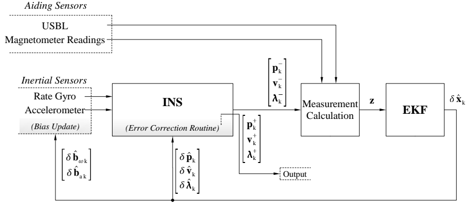
Figure 2: Navigation System Block Diagram
